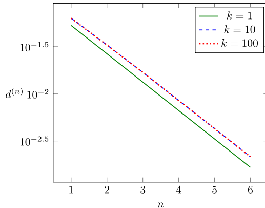
FIGURE 2. Convergence of the relative error of the state vector for (4.1) with f_1 being a Weierstraß function and \omega^{(n)} computed by Sum-Up-Rounding on refined grids indexed by n = 1, \dots, 6 . The cases k = 10 and k = 100 coincide within the figure's resolution.
