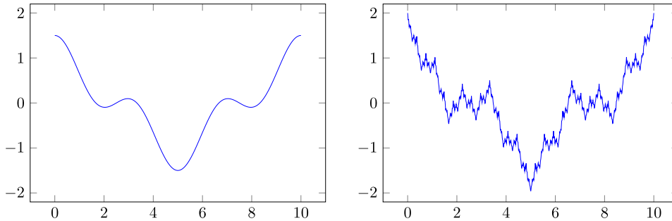
FIGURE 3. Approximants of the Weierstraß function by including one summand ( left ) and ten summands ( right ).
