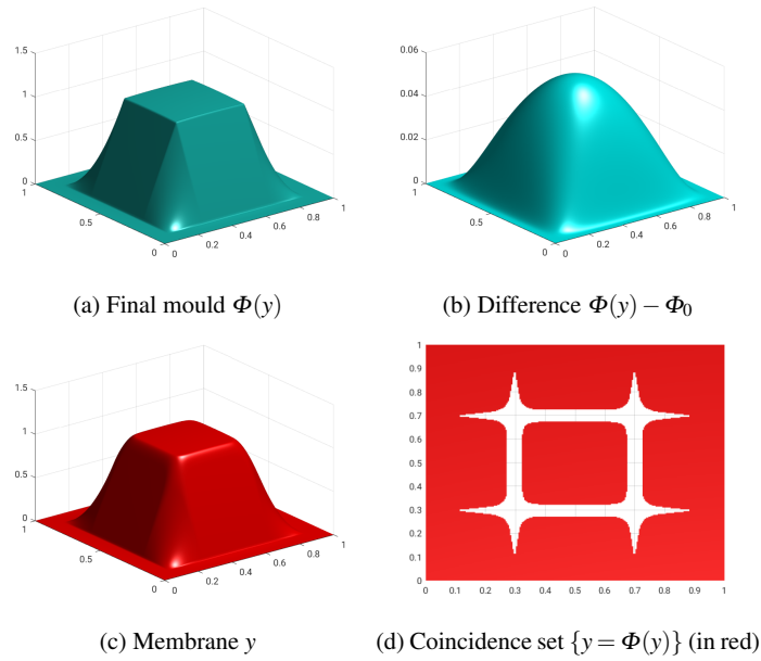
Fig. 1: Results for the thermoforming example
