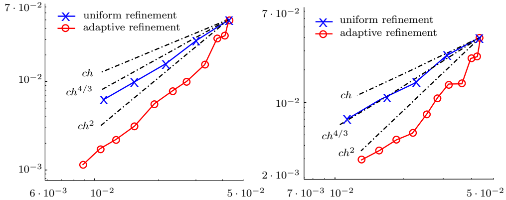
FIGURE 5. Primal-dual gap \delta_h with extrapolated reference value K_{ref} in the modified versions of Examples 6.1 and 6.2.
